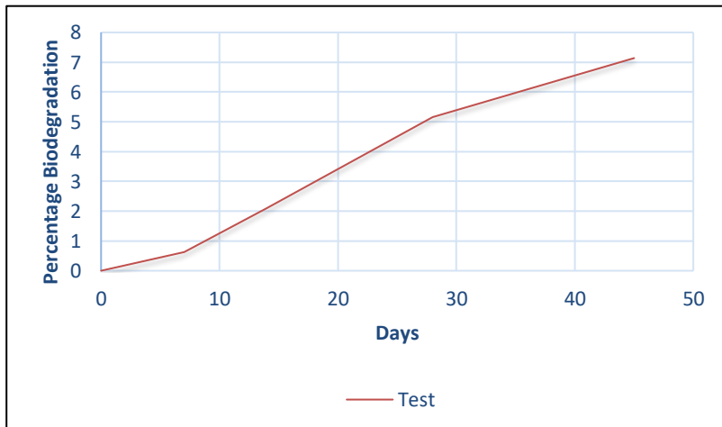
Graph-2b: The percent biodegradation of the Test sample (PBT with 0.5% of BDP– False eyelashes, makeup brushes and shaving brush (0.07*35mm) sample) determined based on conversion of carbon from the Test material to carbon in the gaseous phase (CH 4 and CO 2 )
